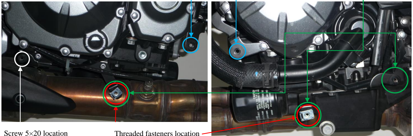
Screw 5×20 location
